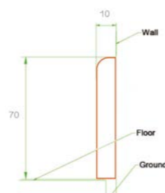
Skirting Rodapié
