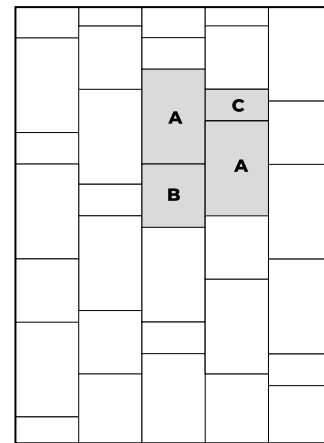
Laying scheme Multisize 2 (random)
